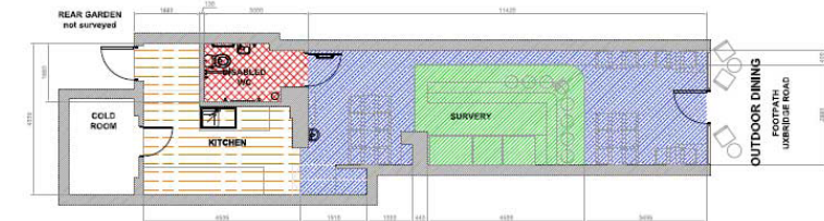
PROPOSED GA PLAN - GROUND FLOOR, OPTION 6 28 COVERS + 4 COVERS OUTSIDE
